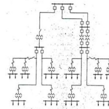
Gambar 1. Sistem Jaringan radial terbuka (Suswanto, 2009)
