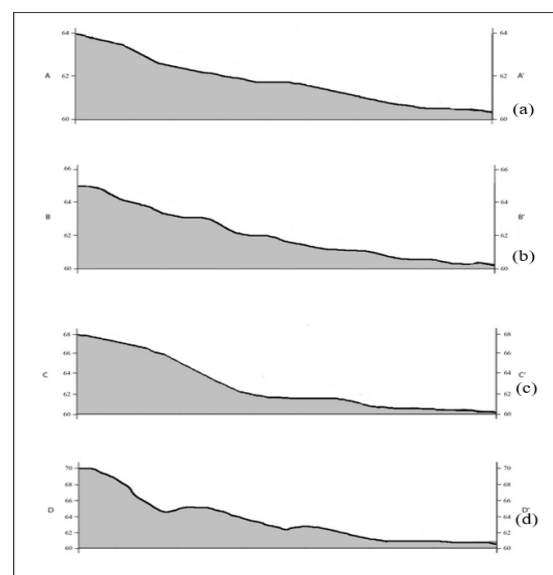
Gambar 5. Penampang cross section jarak 10 m: (a) cross section A-A', (b) cross section B-B', (c) cross section C-C', (d) cross section D-D'
