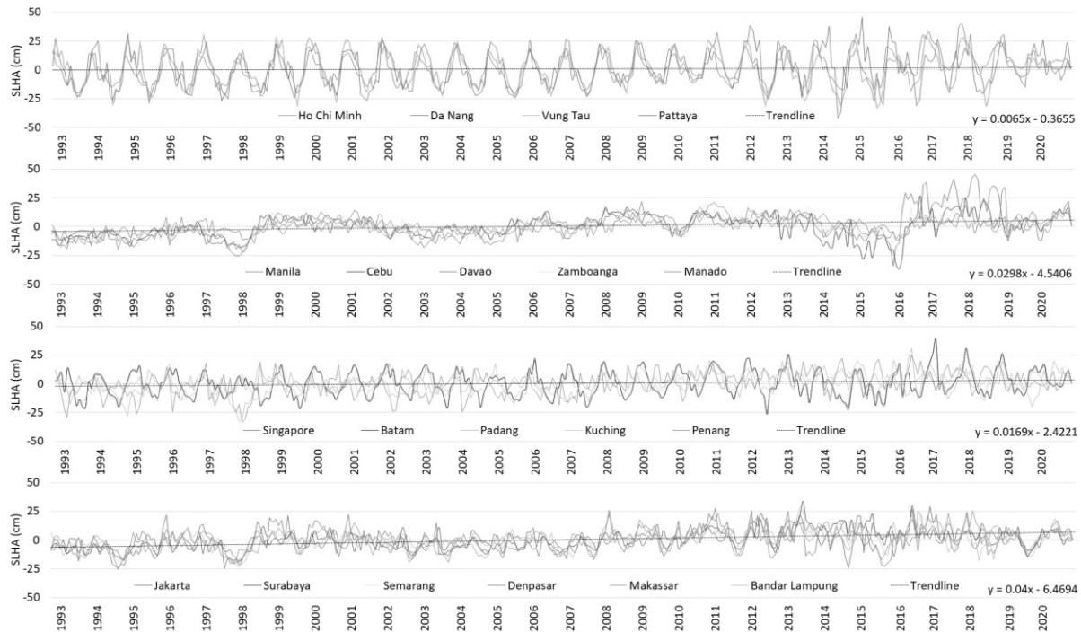
Figure 2. Sea level anomaly trends in Southeast Asia cities during the period of 1992 – 2020.
