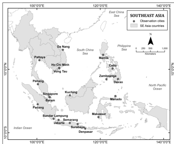
Figure 1. Southeast Asia region and SLR observation cities.
