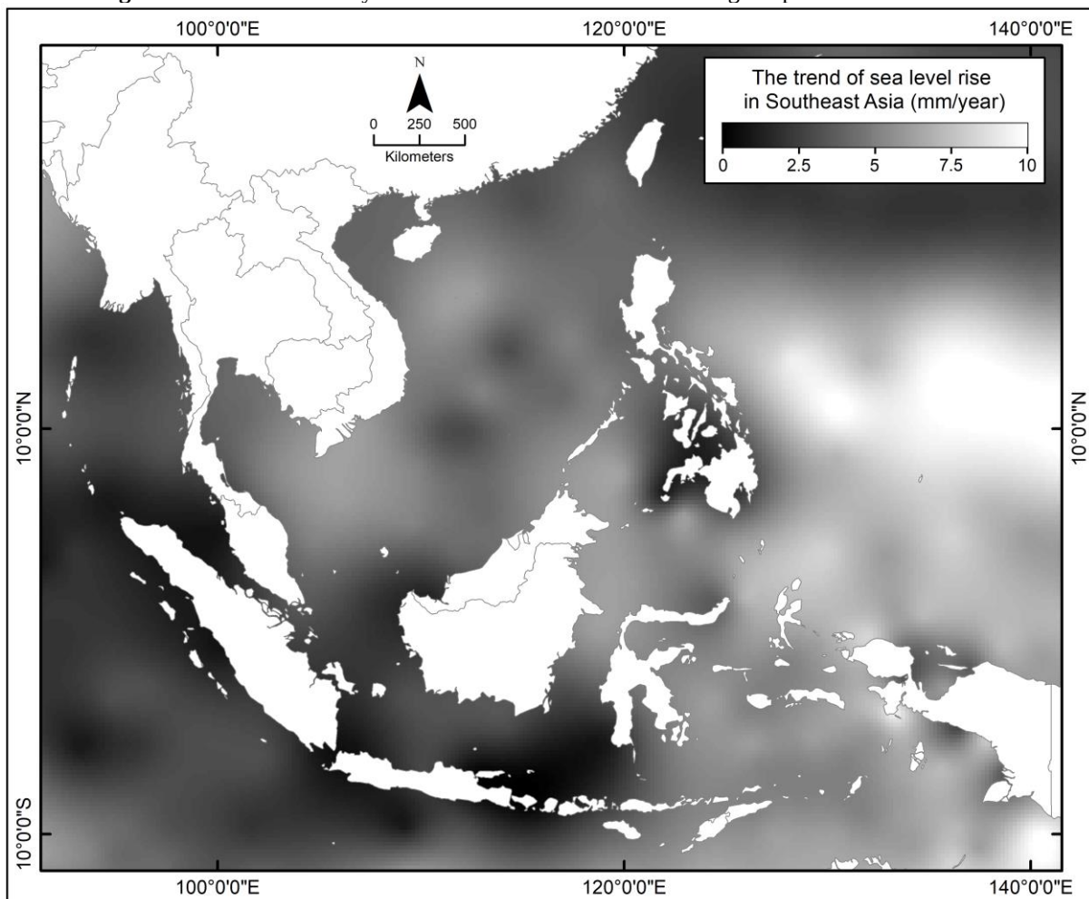
Figure 3. The map of SLR trend based on altimetry satellite data from 1992 – 2020.
